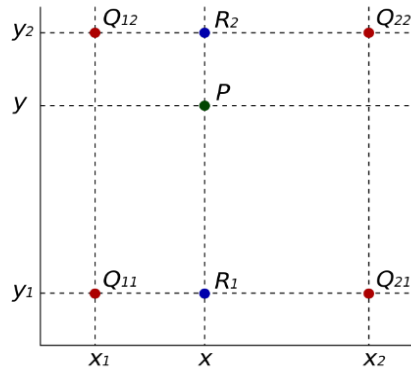
Figure 1. Bilinear resampling to estimate the value f of the point P(x, y) from the point Q_{11} = (x_1, y_1) , Q_{12} = (x_1, y_2) , Q_{21} = (x_2, y_1) , and Q_{22} = (x_2, y_2) .
